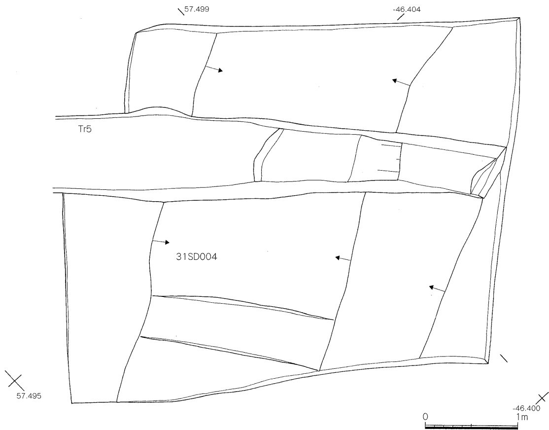
Fig.16 31SD004遺構実測図 (1/40)
