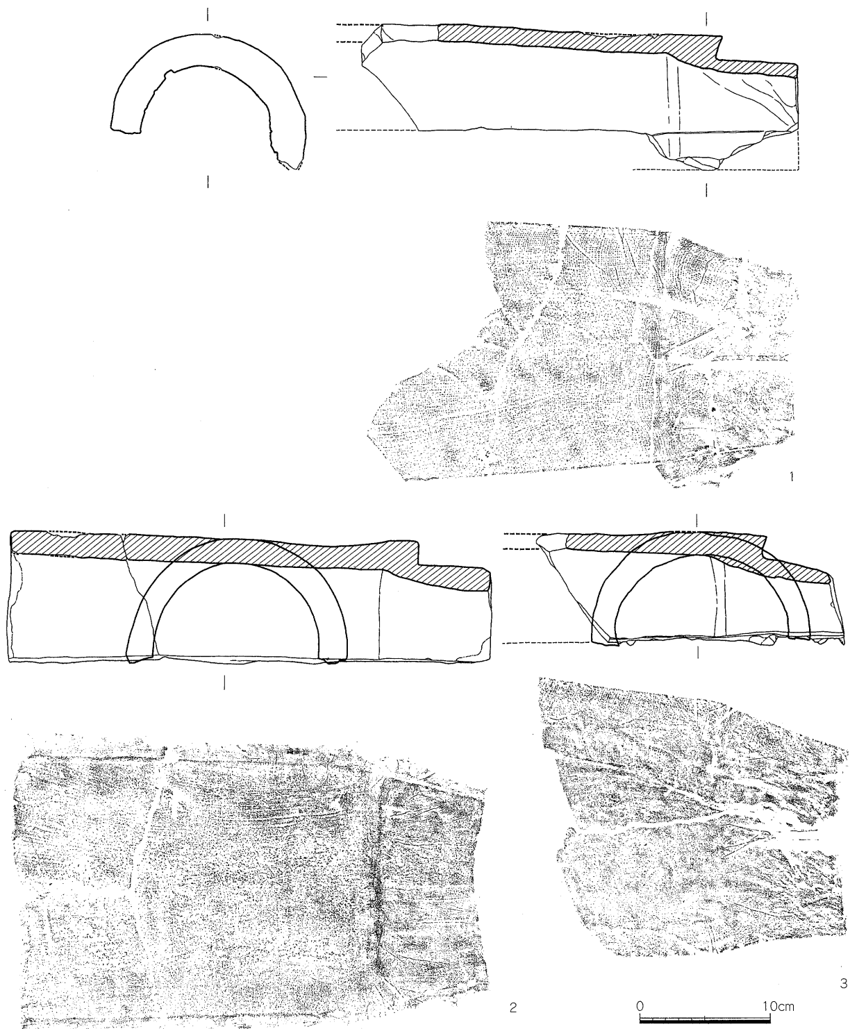
Fig.19 31SX002 (2号瓦窯) 出土遺物実測図1 (1/4)
