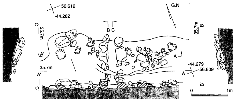
図7.149SX020遺構実測図 (S=1/60)
