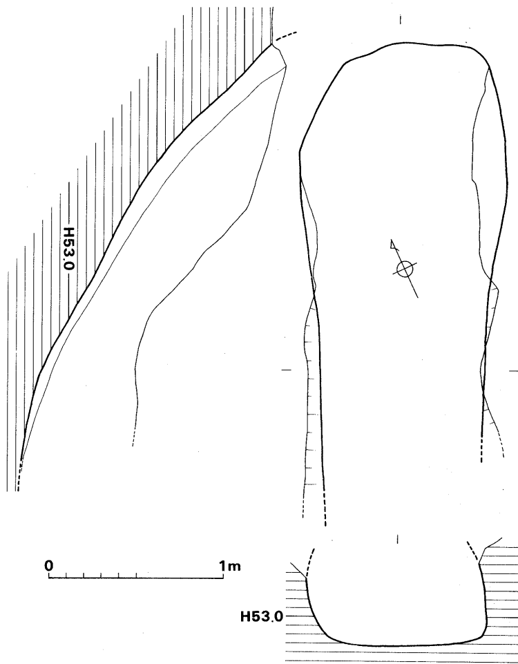
Fig.23 1号窯 (1/30)
