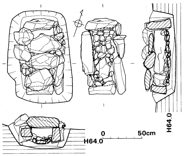
Fig.18 1号石棺墓 (1/30)
