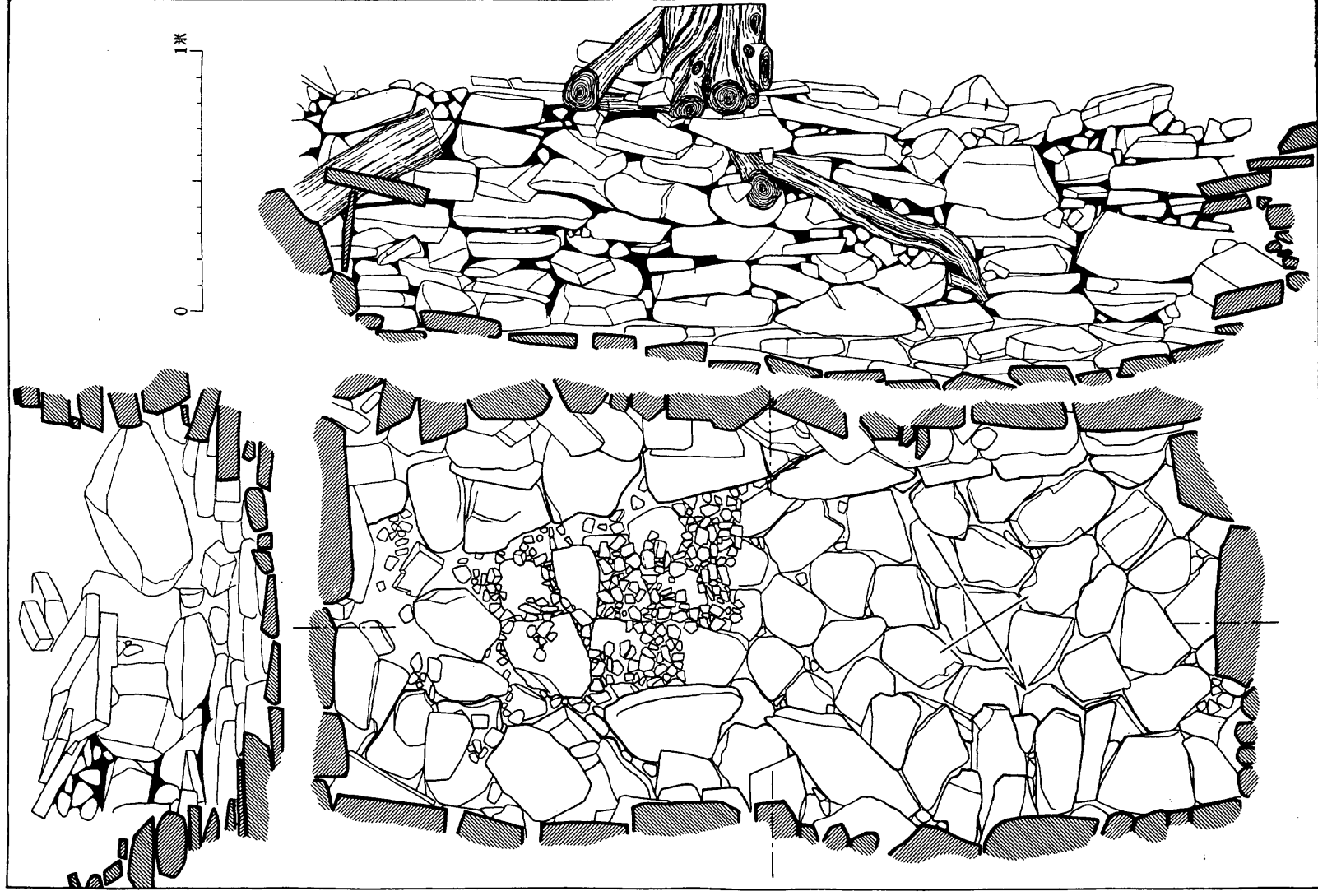
Pl. V. Plan and Section of Interior of the Stone Chamber
